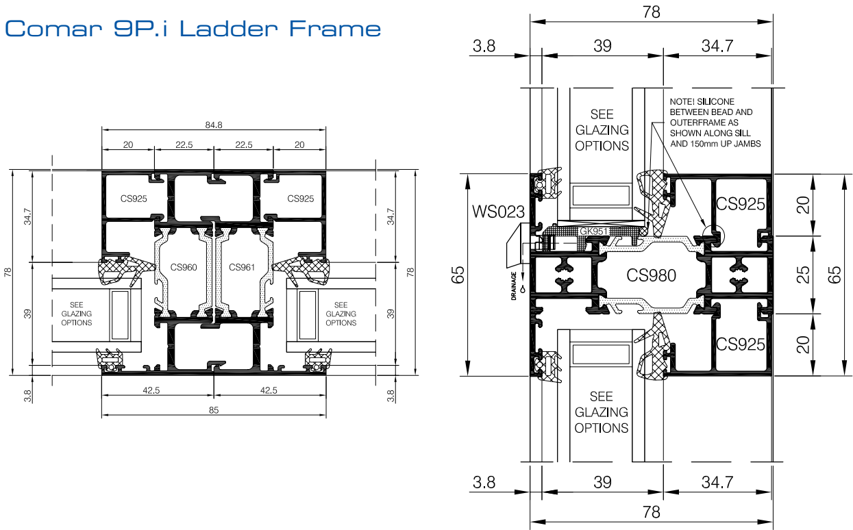
General arrangement showing Comar 9P.i Ladder Frame mullion detail.
